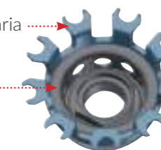
molla secondaria secondary spring
